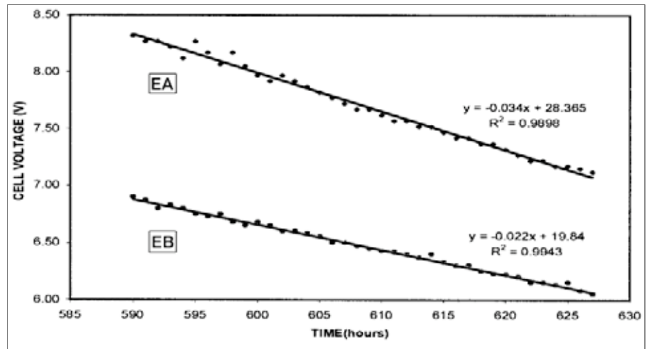
Figure 2. Average cell voltages for Cells A and B, showing the linear decrease in voltages.
