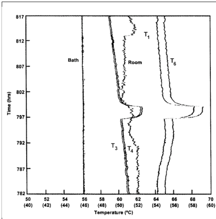
Figure 4. Temperature versus time for Cells A. Thermistors T_1 and T_6 show an anomalous temperature increase for Cell A along with a calibration based on increasing the cell current. Bath and room temperature scales are 20 to 25°C.
