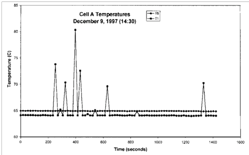
Figure 6. Thermistor readings versus time for Cell A ( T_1 , T_6 ).
